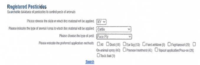
Figure 1: Screenshot of the Veterinary PestX Database dashboard.
